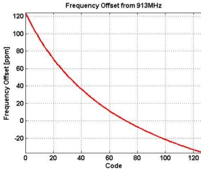
Figure 2. Capacitor Bank Frequency Offset Characteristics
