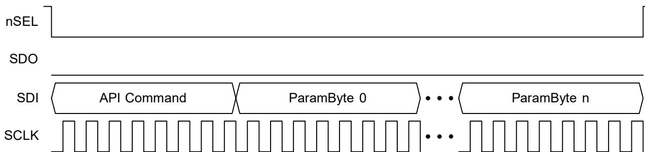
Figure 6. SPI Write Command
