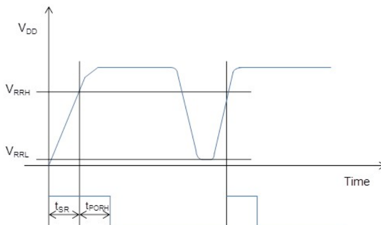
Figure 10. POR Timing Diagram
