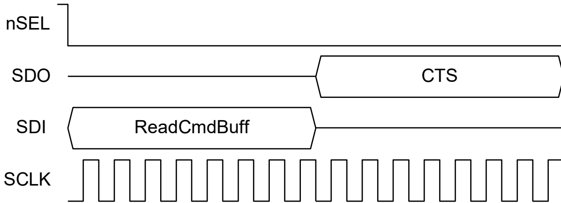
Figure 7. SPI Read Command—Check CTS Value
