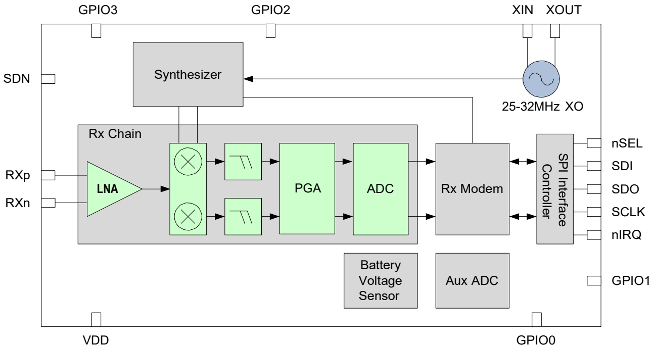
Figure 1. HC4355 Functional Block Diagram
