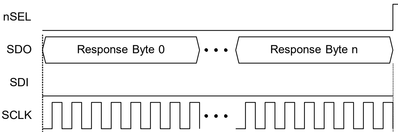
Figure 8. SPI Read Command—Clock Out Read Data
