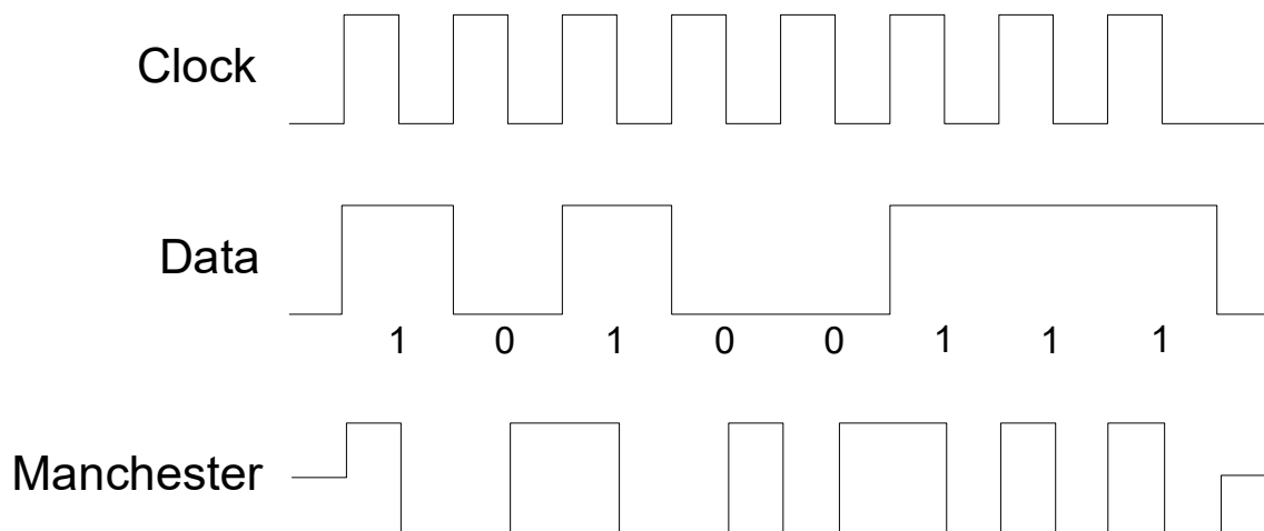
Figure 4. Manchester Code Example
